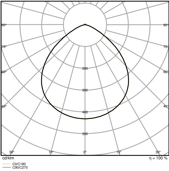
HB DA P 200W 865 110DEG IP66
