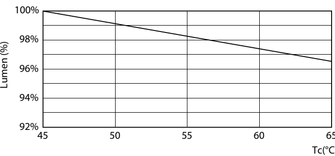
Lumen Maintenance Diagram - CorePro LEDtube HF 1500mm HE 20.5W 865T5
